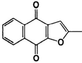
Lapachonone
