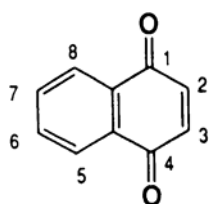
Naphthoquinone
