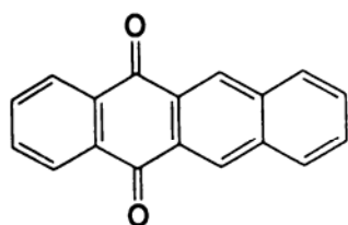
Anthracyclinone
