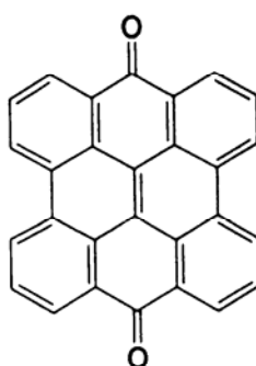
Naphthodianthrone
