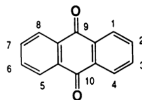
Anthraquinone
